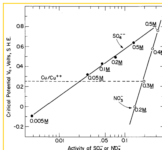
Fig. 6. Critical pitting potentials, determined potentiostatically, of Al in 0.005M NaCl with \text{Na}_2\text{SO}_4 additions, and in 0.1M NaCl with \text{NaNO}_3 additions, 25°C.
