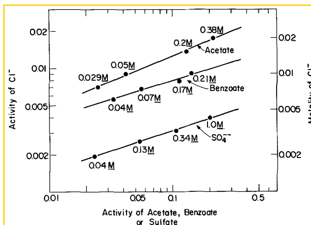
Fig. 3. Relation of minimum activities (or concentrations) of sodium acetate or sodium benzoate or sodium sulfate required to inhibit pitting of 99.99% Al in aerated sodium chloride solutions.
